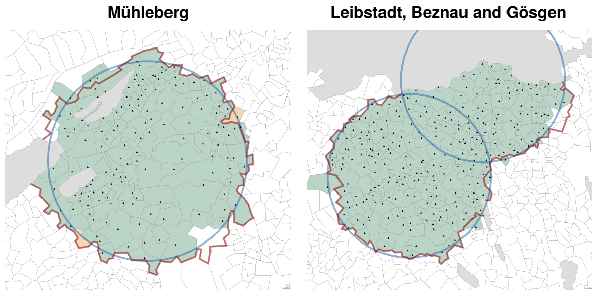
Figure A.2: Reconstructed Assignment Criterion and Observed Iodine Distribution Boundary (2004/05)
