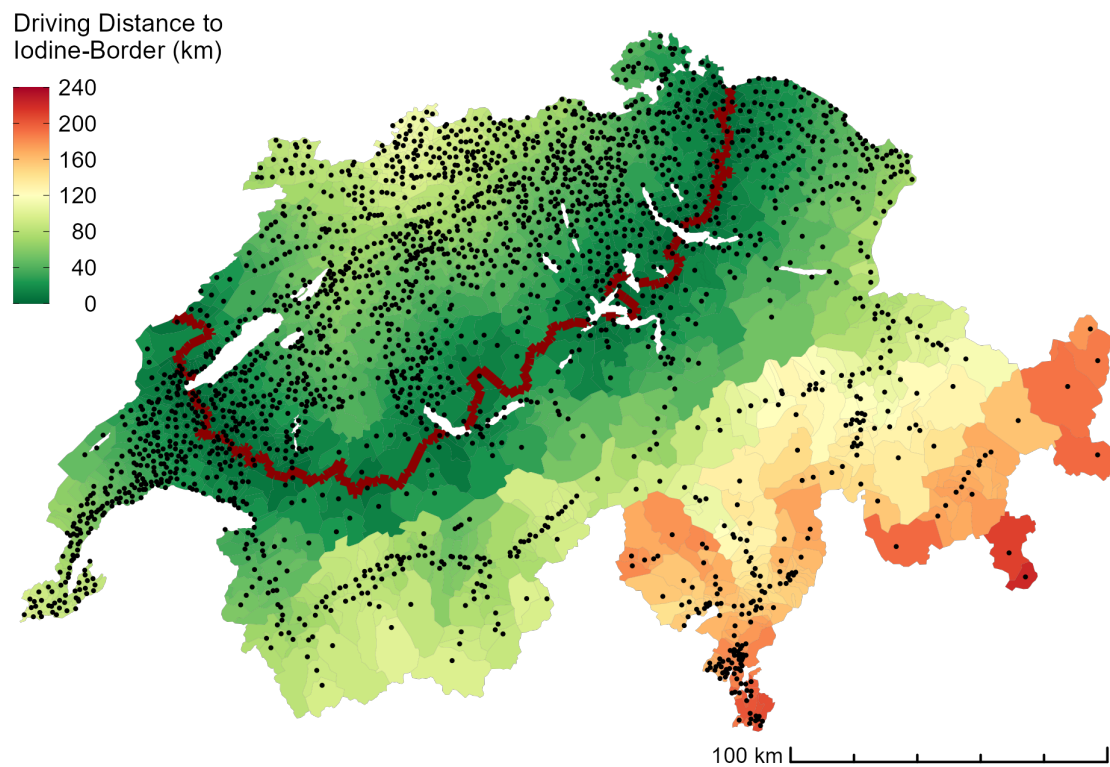
Figure A.1: Driving Distance from every municipality to the iodine boundary 2014/15
